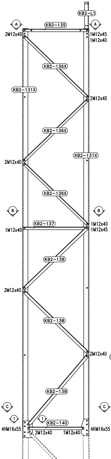
SECTION 1-1
