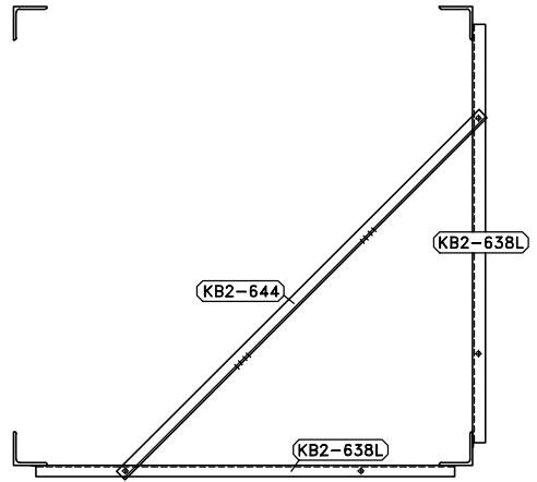
SECTION L1-L1
