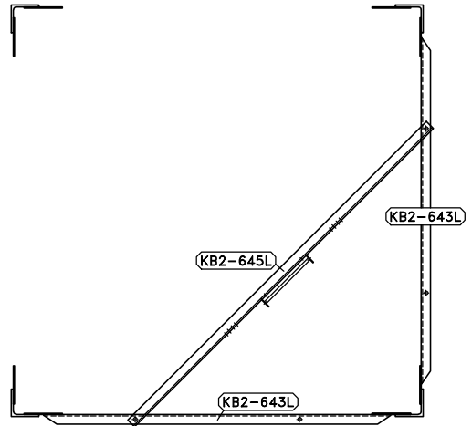
SECTION M1-M1
