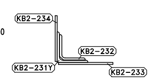
SECTION 2-2
