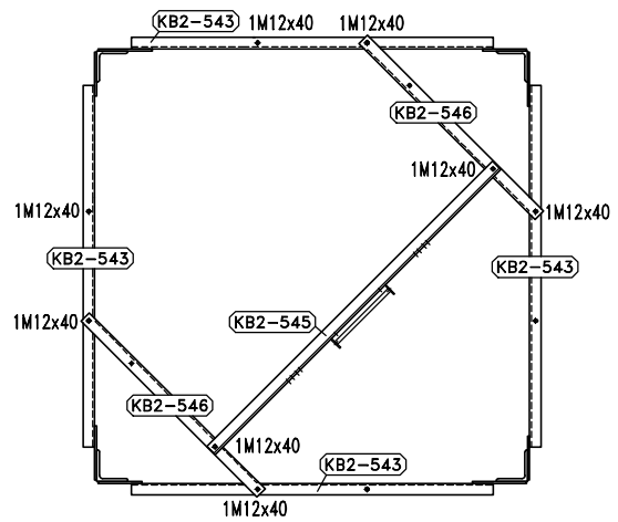
SECTION K-K
